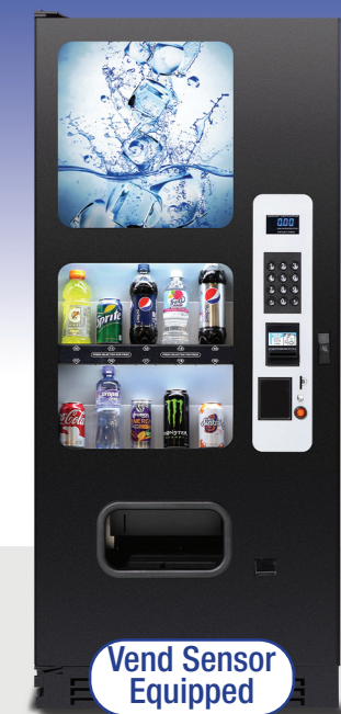
AB10/500 Bottle & Can Vendor 72" x 31.75"W x 36.5"D, *Ship Weight 671 lbs / 10 Selections Capacity: 500 - 12 oz Cans or 240 - 20 oz Bottles or a Combination Standard Vend Sizes 12 oz, 16.9 oz, 20 oz & 24 oz (Optional kit needed for 250 ML energy drink cans) Card reader available
